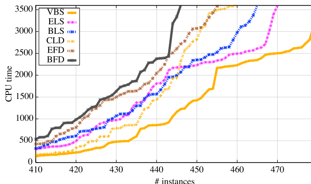
Figure 2: Cactus plot for enumerating all MCSes
